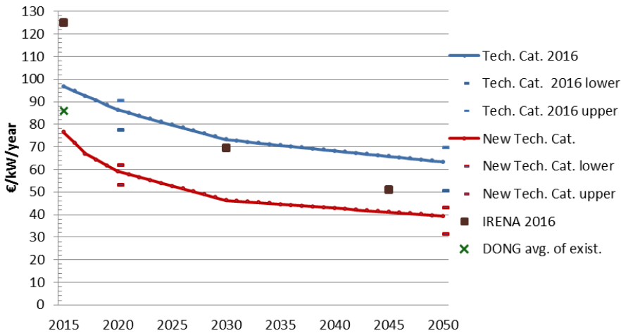
Figure 2: OPEX total annual with annual production equal to expected full load hours (FID year).
