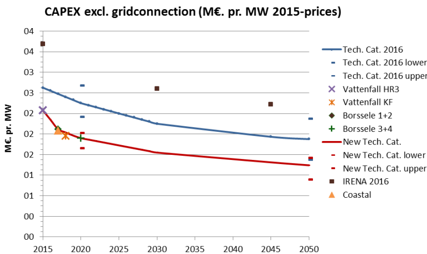
Figure 1: CAPEX excl. grid connection (FID year)
