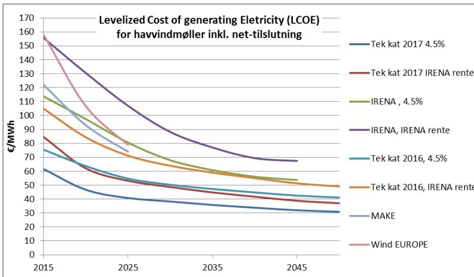
Figure 3: Own calculations of the LCOEs for the Technology Catalogue and IRENA data applying different interest rates (WACC). Note 1: It has been assessed that MAKE and Wind Europe have applied an interest rate of 4-5% when calculating the LCOEs.
